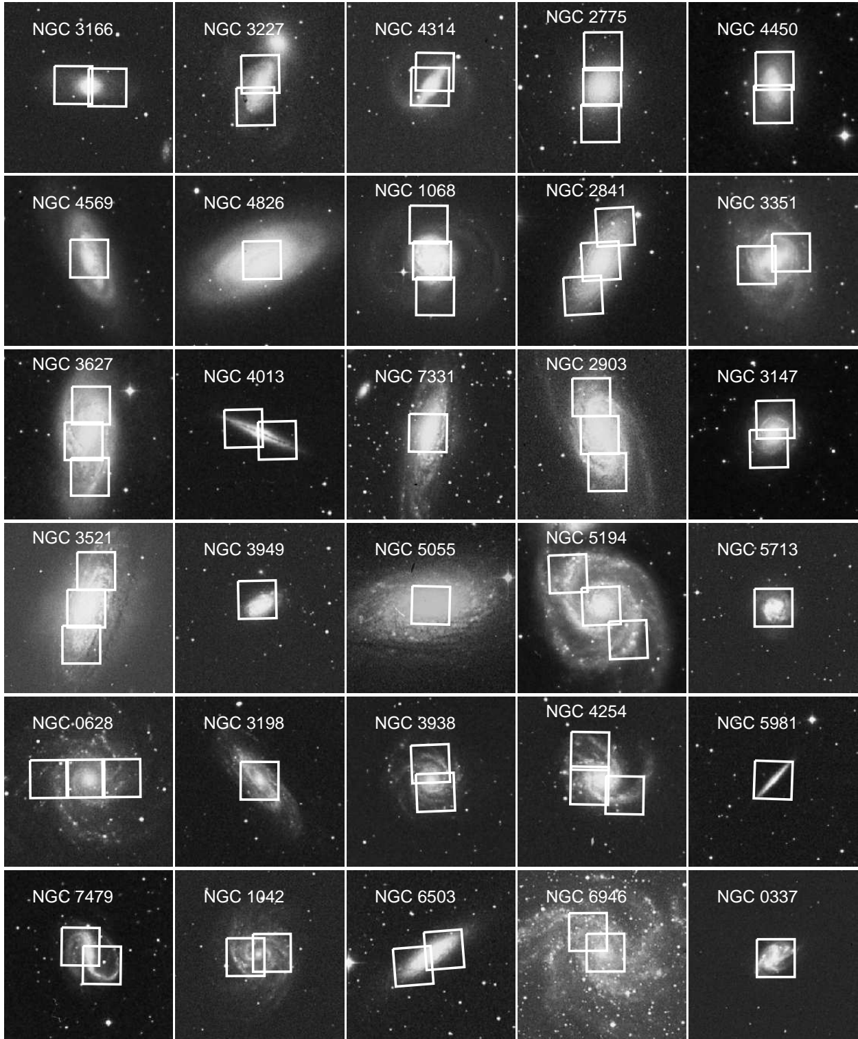
Fig. 1.— Digital Sky Survey cutouts of the 30 galaxies in the VENGAs sample. The targets are ordered by Hubble type (taken from RC3, de Vaucouleurs et al. (1991)) from earlier to later. White boxes show the VIRUS-P 1.7' \times 1.7' pointings observed on each galaxy.
