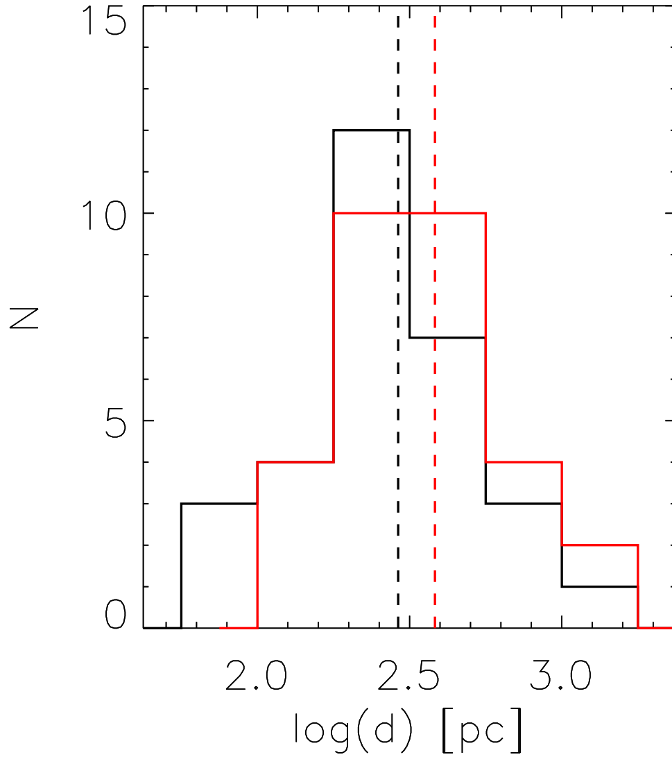
Fig. 3.— Histogram of the logarithm of the VIRUS-P 4.24'' fiber size in physical units for each galaxy in the VENGAs sample (black), given the distances adopted in Table 1. Also shown is the size of the 5.6'' FWHM PSF of the final data-cubes (red). The vertical dashed lines mark the median native and effective spatial resolutions of 290 pc and 383 pc.
