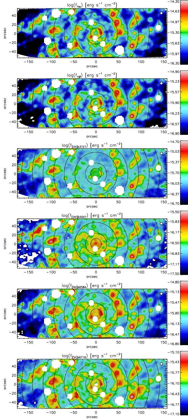
Fig. 13.— Maps of NGC 628 in different emission lines. From top to bottom: H\alpha , H\beta , [OII]\lambda 3727 , [OIII]\lambda 5007 , [NII]\lambda 6584 , and [SII]\lambda 6716 . Black contours show lines of constant galactocentric radii spaced by 1 kpc, with the exception of the innermost contour at a radius of 0.5 kpc. Spaxels contaminated by foreground MW stars (see §6.1) are masked.
