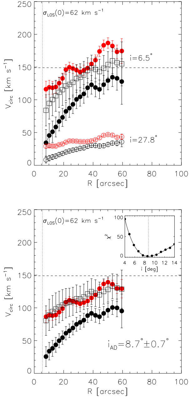
Fig. 18.— Top Panel: Stellar (black) and ionized gas (red) rotation curves for NGC 628 under the assumption of two different inclination values of 6.5^\circ (filled circles) and 27.8^\circ (open circles). Open squares show the stellar rotation curve after applying the asymmetric drift correction for the i = 6.5^\circ case. The horizontal dashed line marks the asymptotic rotation velocity of 149 \text{ km s}^{-1} expected from the Tully-Fisher relation. The size of the VENGA PSF FWHM is marked by the dotted vertical line. Lower Panel: Same as above, but for the best-fit asymmetric drift inclination ( i_{\text{AD}} = 8.7^\circ \pm 0.7^\circ ). The inset shows the \chi^2 distribution for the range of inclination values explored during the fit. The vertical dotted line in the inset marks the best-fit inclination.
