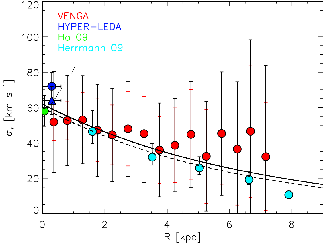
Fig. 17.— Radial profile of \sigma_* = \sigma_{LOS} . Red circles mark the median \sigma_* for all spaxels in 0.5 kpc wide radial bins. Error bars show both the standard deviation in each radial bin (red) and the median error in \sigma_* for each spaxel (black). The central stellar velocity dispersion values from HyperLeda and Ho et al. (2009) are shown in blue and green respectively. The dispersion profile measured by Ganda et al. (2006) using the SAURON IFU spectroscopy is shown as a black dashed curve. The velocity dispersion profile measured from PN kinematics by Herrmann et al. (2008) is also shown (light blue circles, dashed line). The solid black curve shows the best-fit dispersion profile used to calculate the asymmetric drift correction.
