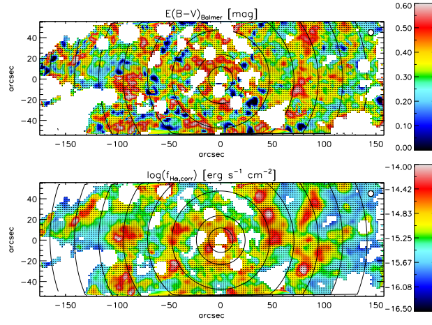
Fig. 14.— Upper Panel: Map of the dust reddening E(B - V) computed using Equation 4. Regions where the uncertainty in E(B - V) is larger than 0.2 mag have been masked. These masked regions correspond mainly to low surface brightness parts of the galaxy where the \text{H}\alpha to \text{H}\beta ratio cannot be measured with high S/N . Lower Panel: Map of the \text{H}\alpha emission line flux corrected for the effects of dust extinction using a MW extinction law. Black contours are as in Figure 13. Spaxels contaminated by foreground MW stars (see §6.1) are masked in both panels.
