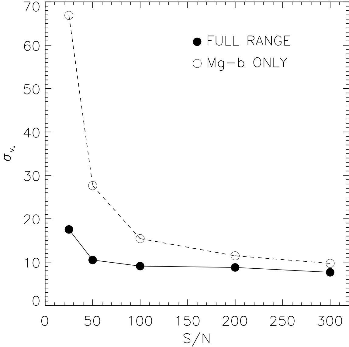
Fig. 11.— Error (standard deviation) in the recovered stellar velocity for fits to simulated spectra with \sigma_{*,true} < 100\text{km s}^{-1} as a function of signal-to-noise ratio. Filled and open circles correspond to fits using the full spectral range and fits limited to the 5100Å–5300Å window respectively.
