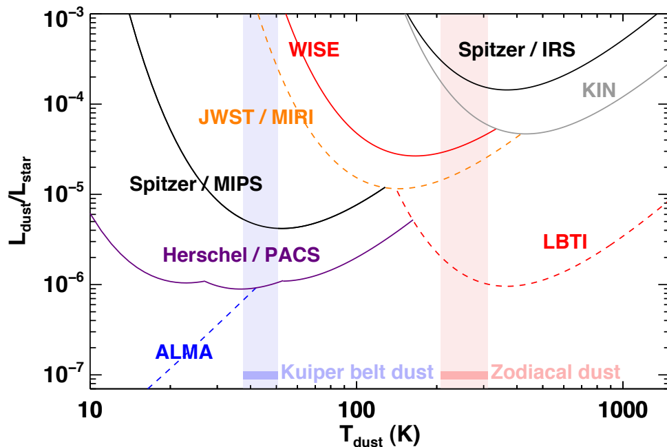
Figure 25: Taken from Roberge et al. (2012). Fig. 3. Sensitivity limits for detection of debris dust around nearby Sun-like stars, for various recent (Spitzer, WISE), current (KIN, Herschel) and near-term facilities (LBTI, JWST, ALMA). The curves show 3\sigma detection limits in terms of the fractional dust luminosity ( L_{dust}/L_{star} ) versus its temperature. Recent and current facilities are plotted with solid lines, near-term ones with dashed lines. The temperature ranges for dust in two zones around the Sun are shown with vertical bars, calculated assuming blackbody grains. The habitable zone (0.8 AU – 1.8 AU) is shown in pink, the Kuiper belt (30 AU – 55 AU) is shown in light blue. The modeled L_{dust}/L_{star} values for the Solar System’s Kuiper belt dust are marked with horizontal light blue and pink bars. An optimized coronagraph on the NRO telescope could be sensitive to L_{dust}/L^* \sim 10^{-6} at T_{dust} \sim 200 K.
