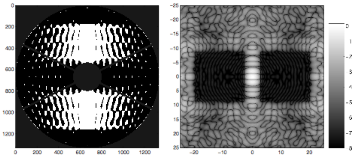
Figure 21: A shaped pupil (left) designed for a pupil similar to the NRO telescope pupil with central obstruction and the corresponding high-contrast point spread function (right). Dark holes are 10^{-8} contrast with an inner working angle of 3 \lambda/D (0.2 arcsec at 800 nm) and an outer working angle of 21 \lambda/D .
