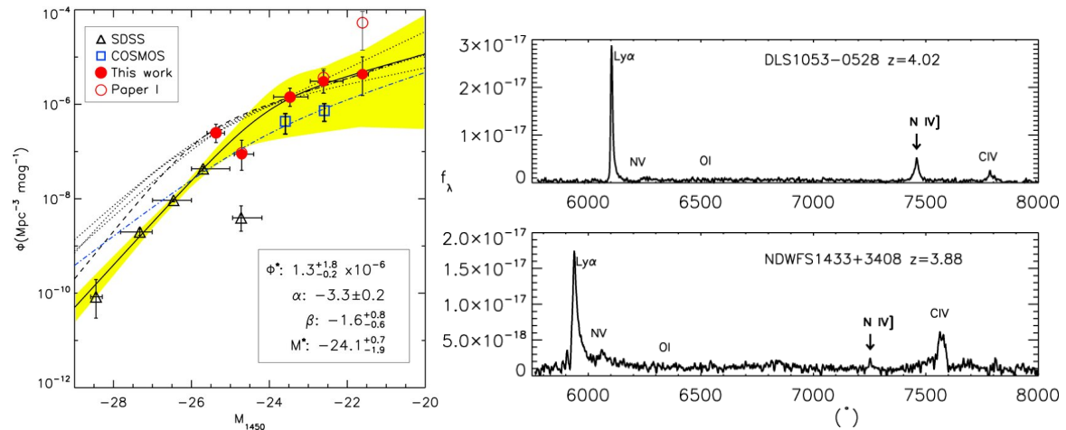
Figure 13: [From Glikman et al. 2007] (left) QSO luminosity function (QLF) at z \sim 4 , combining data from SDSS (triangles), COSMOS (blue squares; Ikeda et al. 2011) and the Bootes field (filled red circles; Glikman et al. 2011). Note the similar faint end slopes but differing normalizations for the latter two. The solid line shows the best-fit double power law; parameters listed in lower right. [From Glikman et al. (2011).] (right) Keck-LRIS spectra of two faint QSOs at z \sim 4 with unusually strong N IV] 1486 emission. This emission line is very rare in bright QSO samples such as in the SDSS, but appears in \sim 9\% of faint quasars at z \sim 4 in the study of Glikman et al. (2007).
