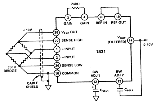
Figure 3. Narrow Bandwidth Application
