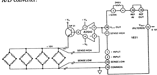
Figure 17. Multiple Load-Cell Application
